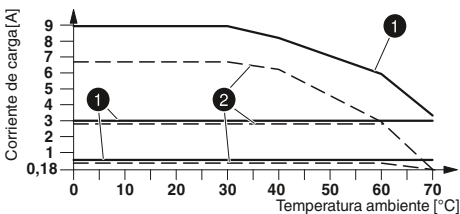
Curva derating
